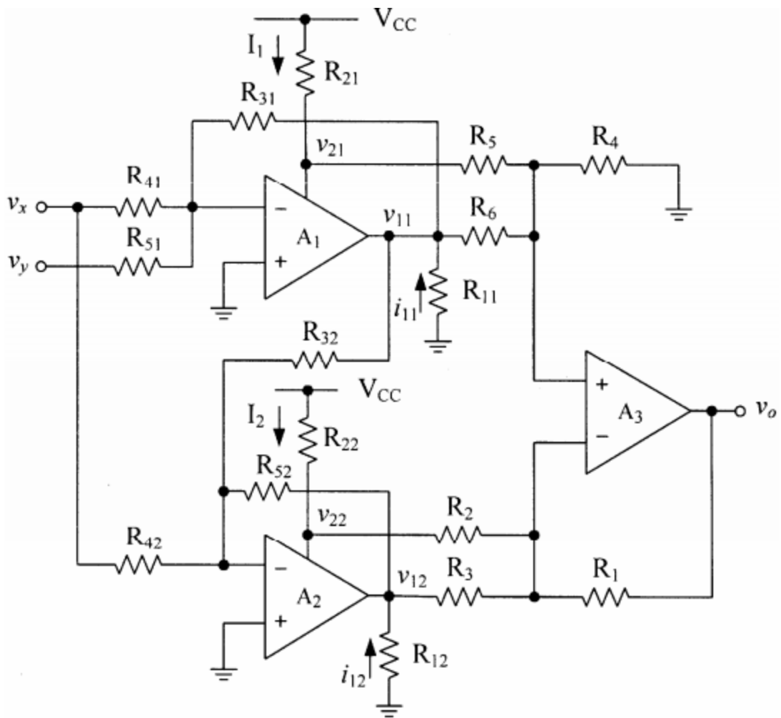
Fig: Analog multiplier using operational amplifier
