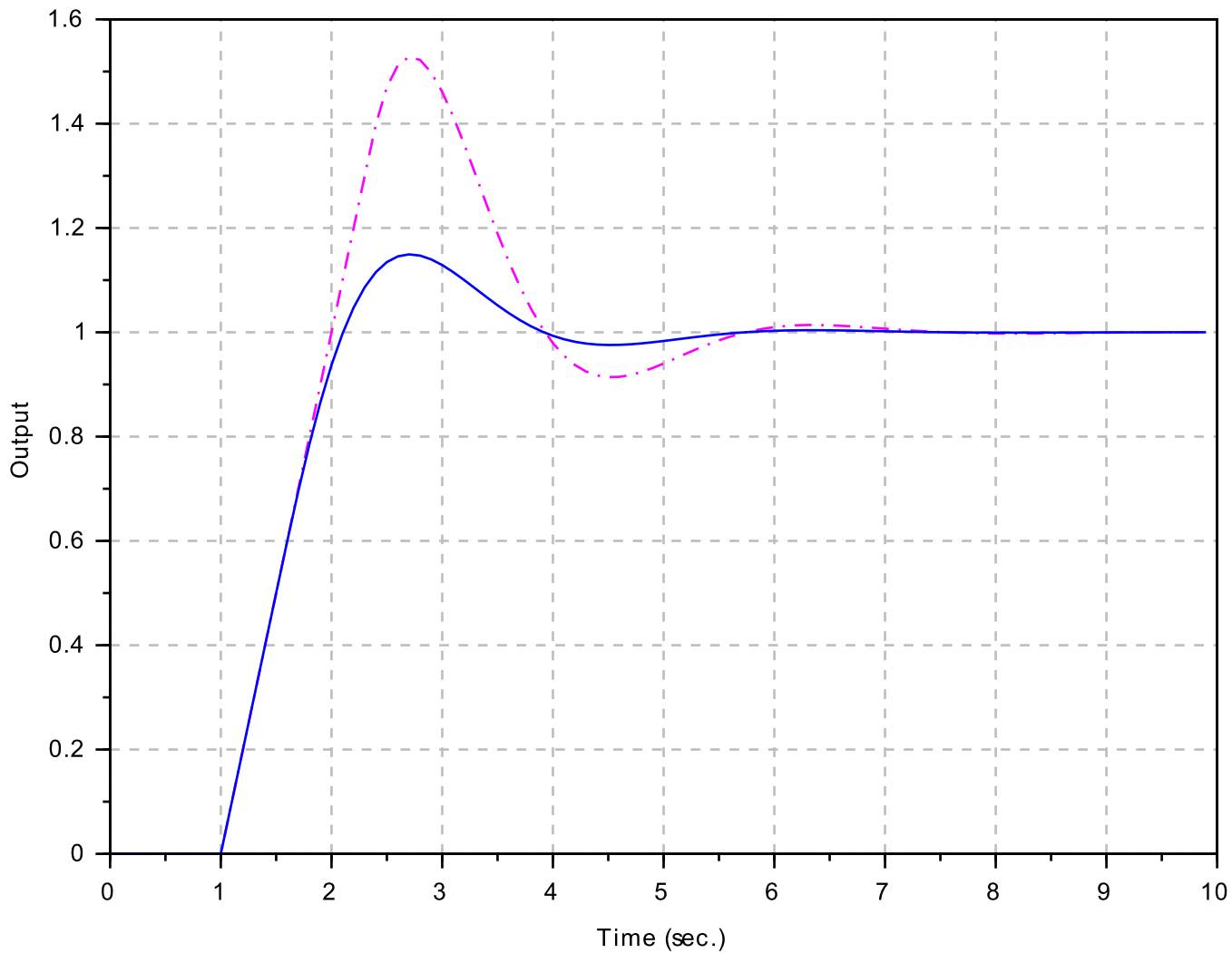
Integrator antiwindup (a) step response.
