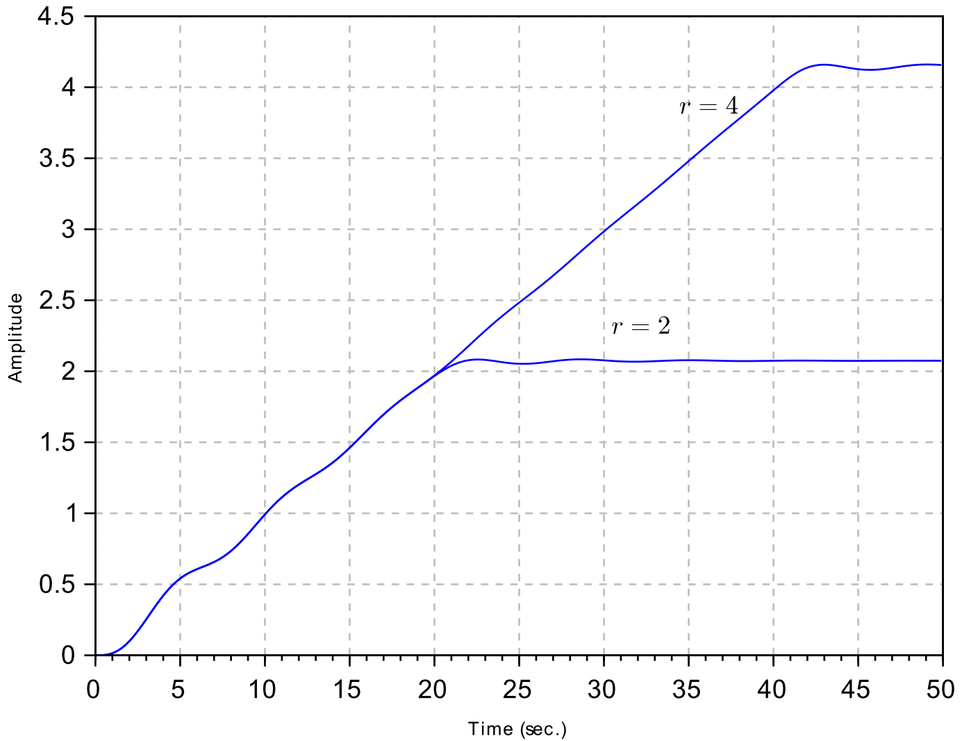
Step response of the system with notch filter
