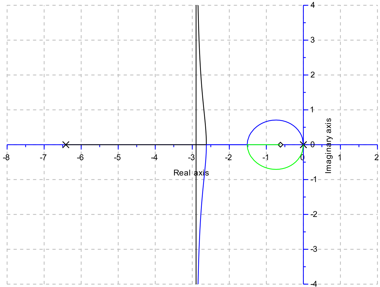
Root locus of a reduced order controller and 1/s^2 process
