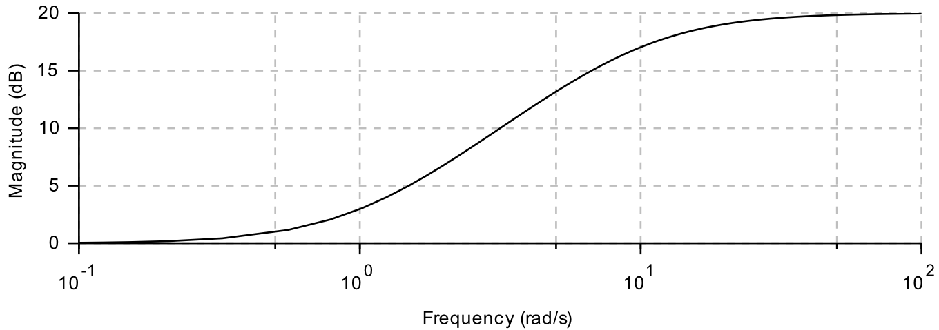
(a) Magnitude and (b) phase for the lead compensator
