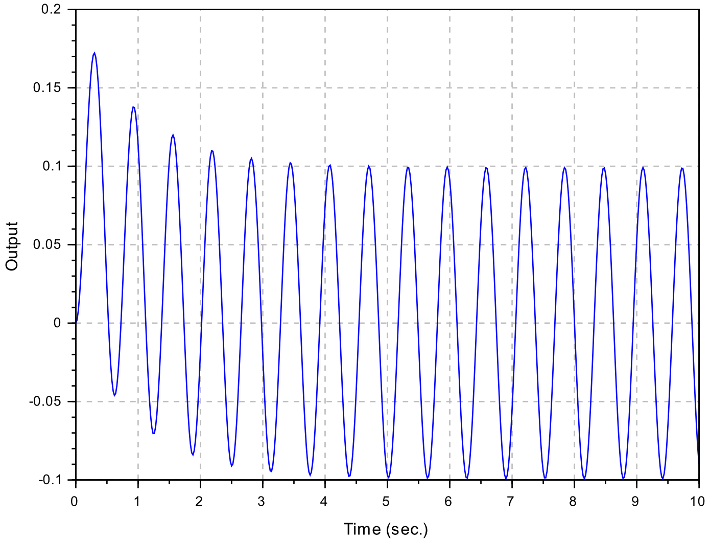
Complete transient response
