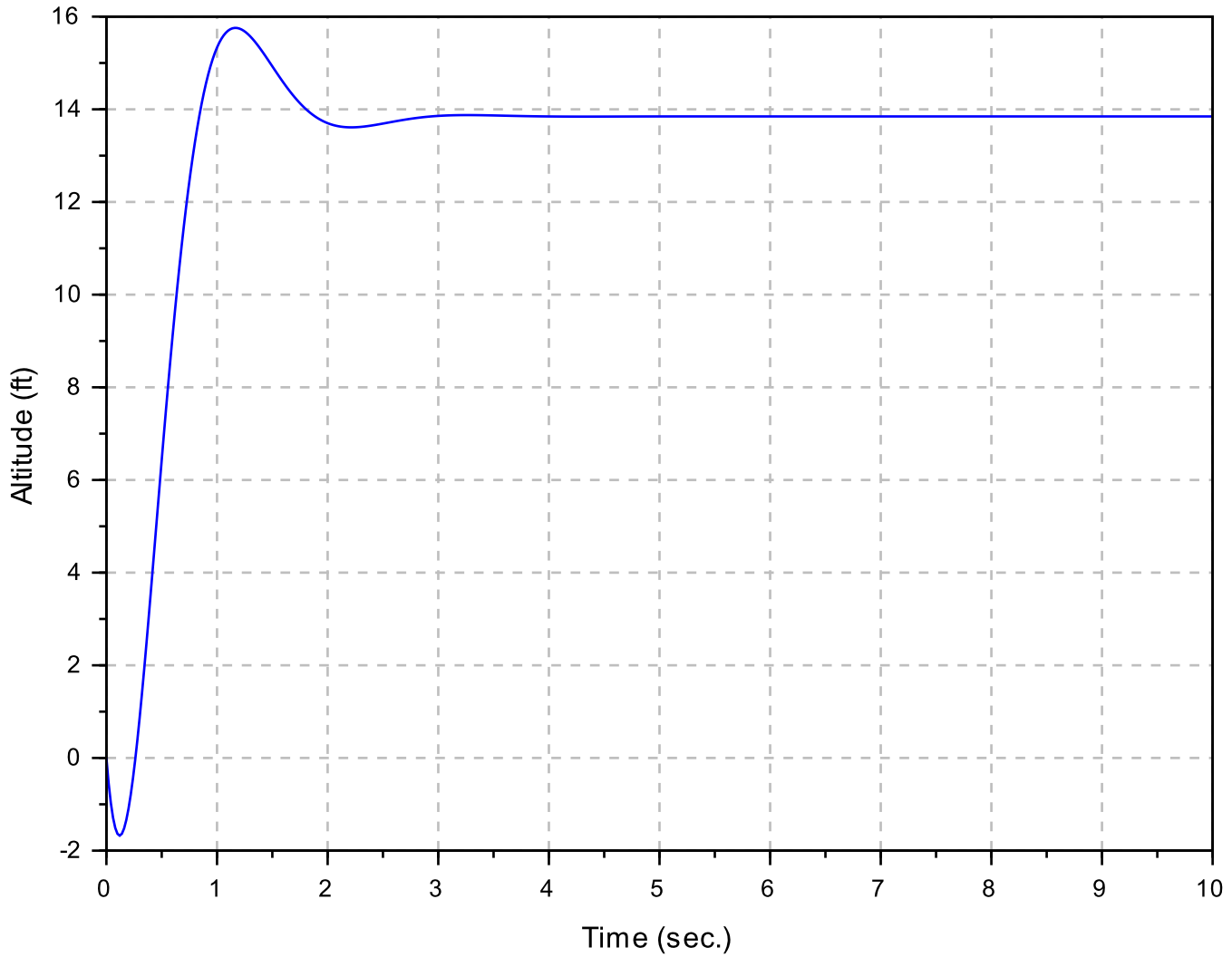
Response of an airplanes altitude to an impulsive elevator input
