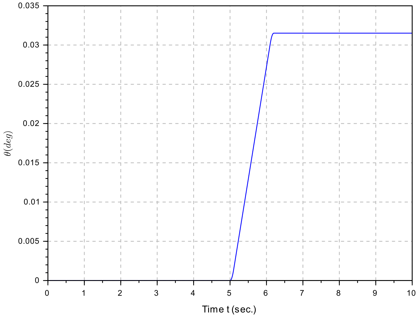
Transient response of the satellite(double-pulse) (b) satellite attitude
