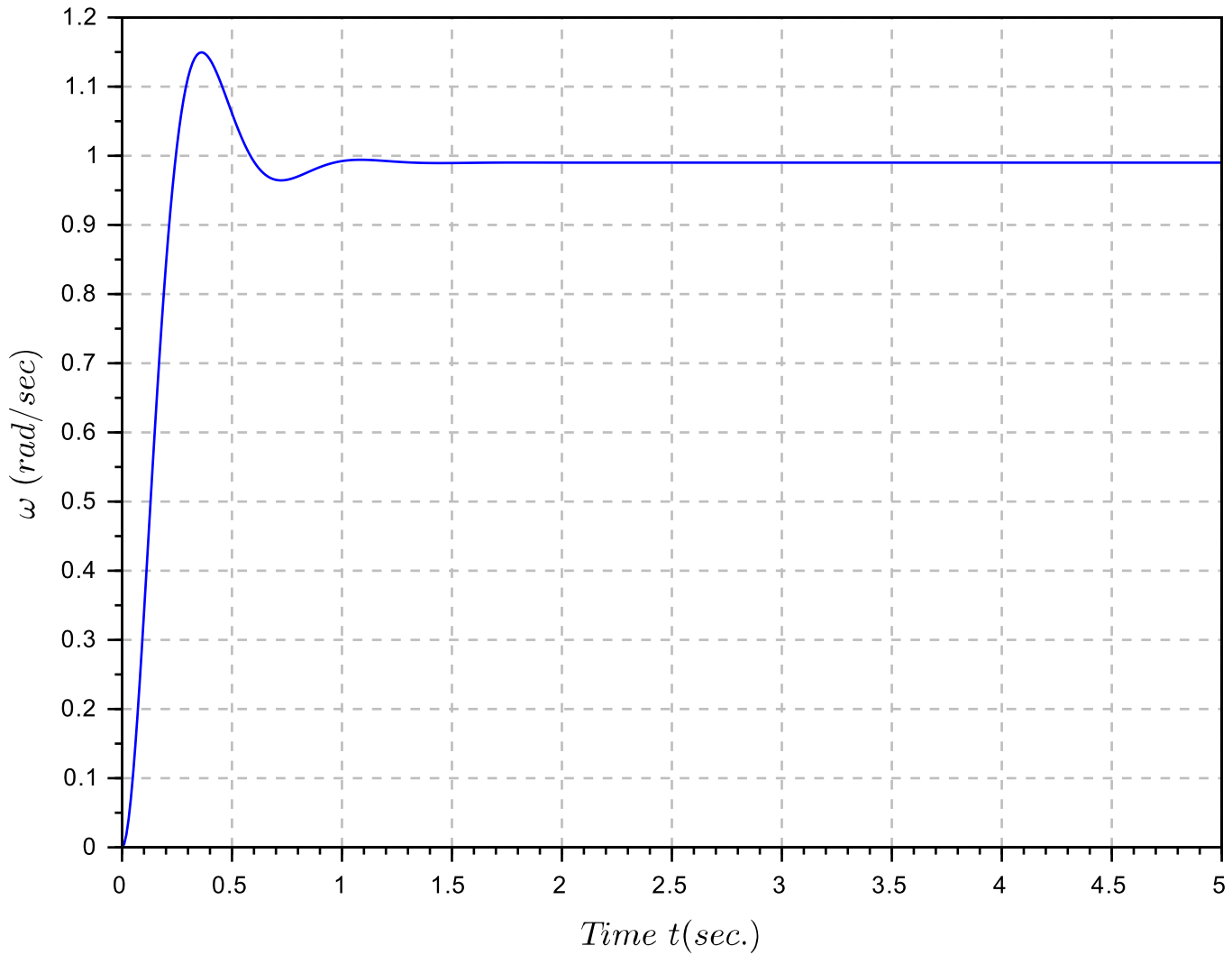
Transient response of DC Motor
