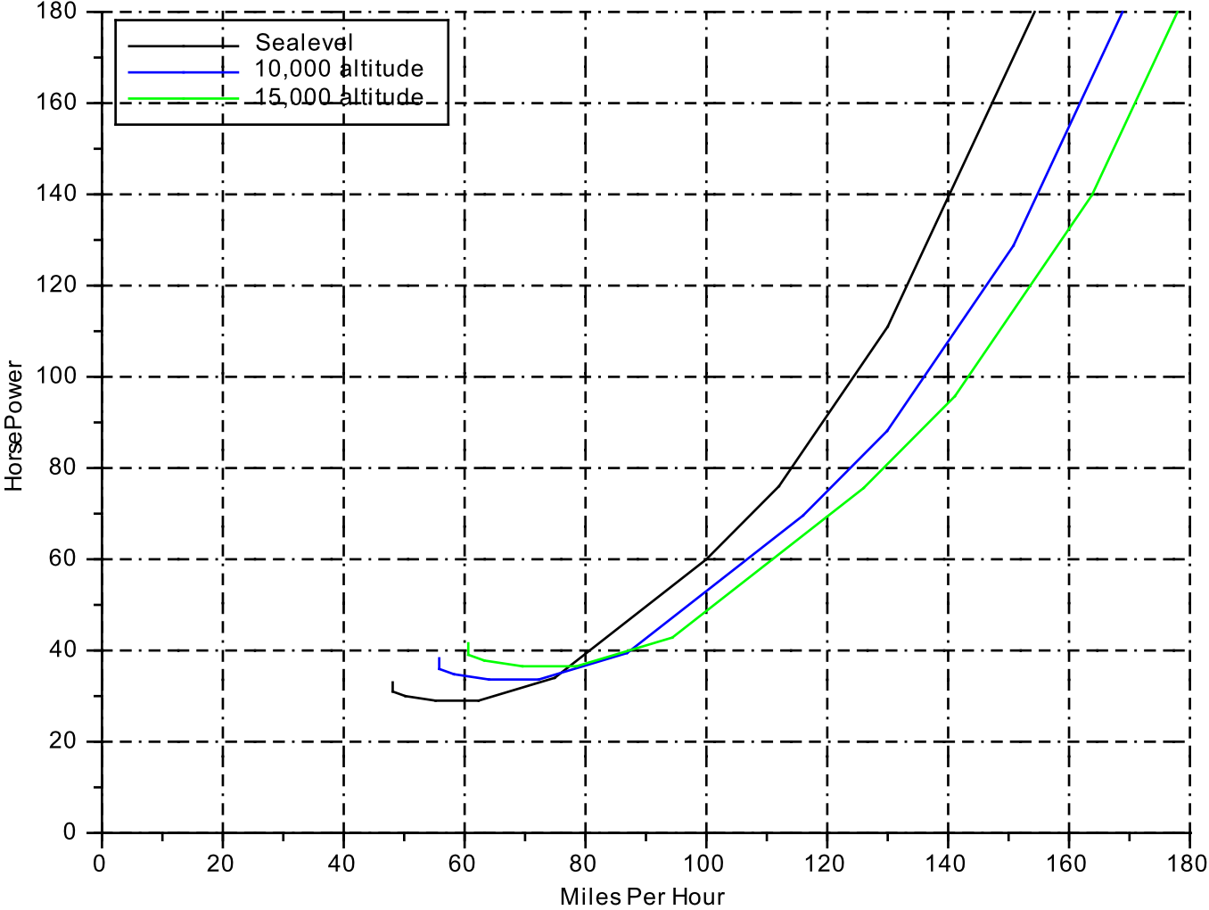
Power Curves
