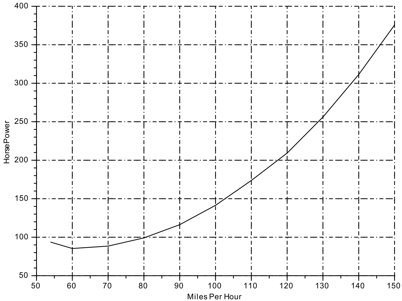
Horsepower required for various airspeeds
