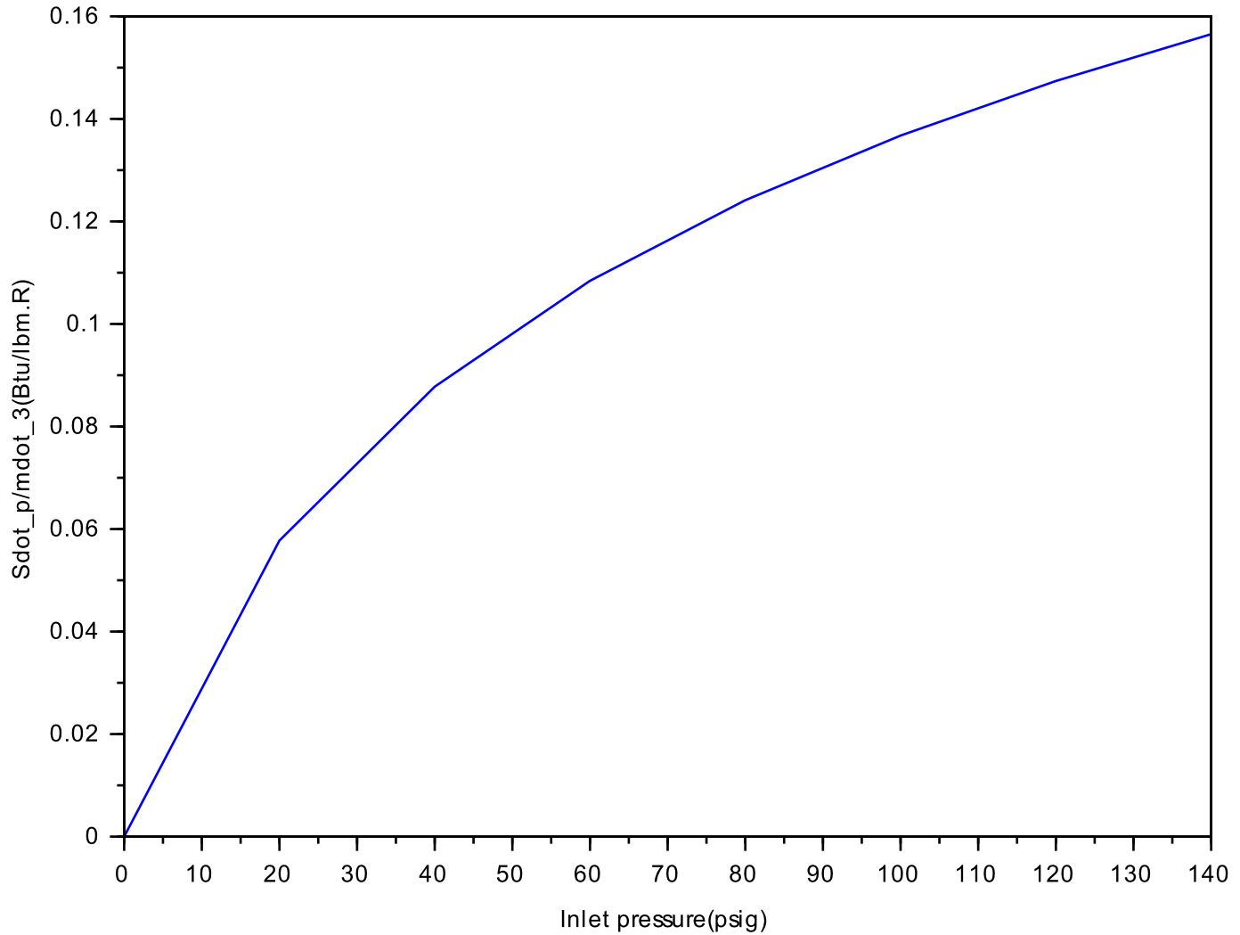
Sdot_p/mdot_3 vs. inlet pressure for a vortex tube
