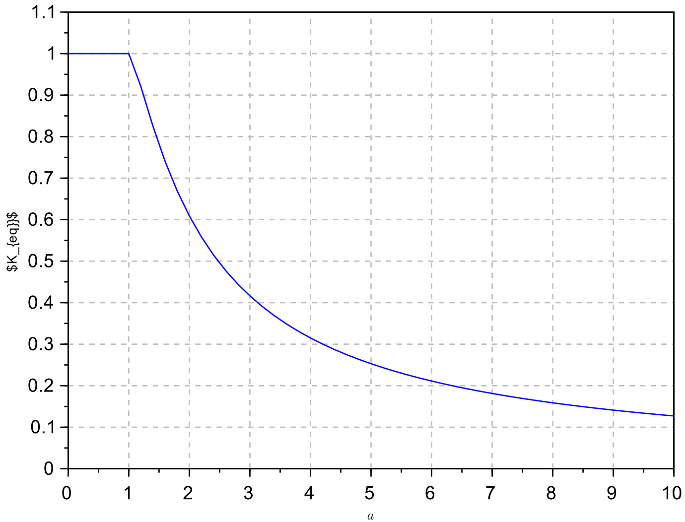
Describing Function for a saturation nonlinearity with k=N=1
