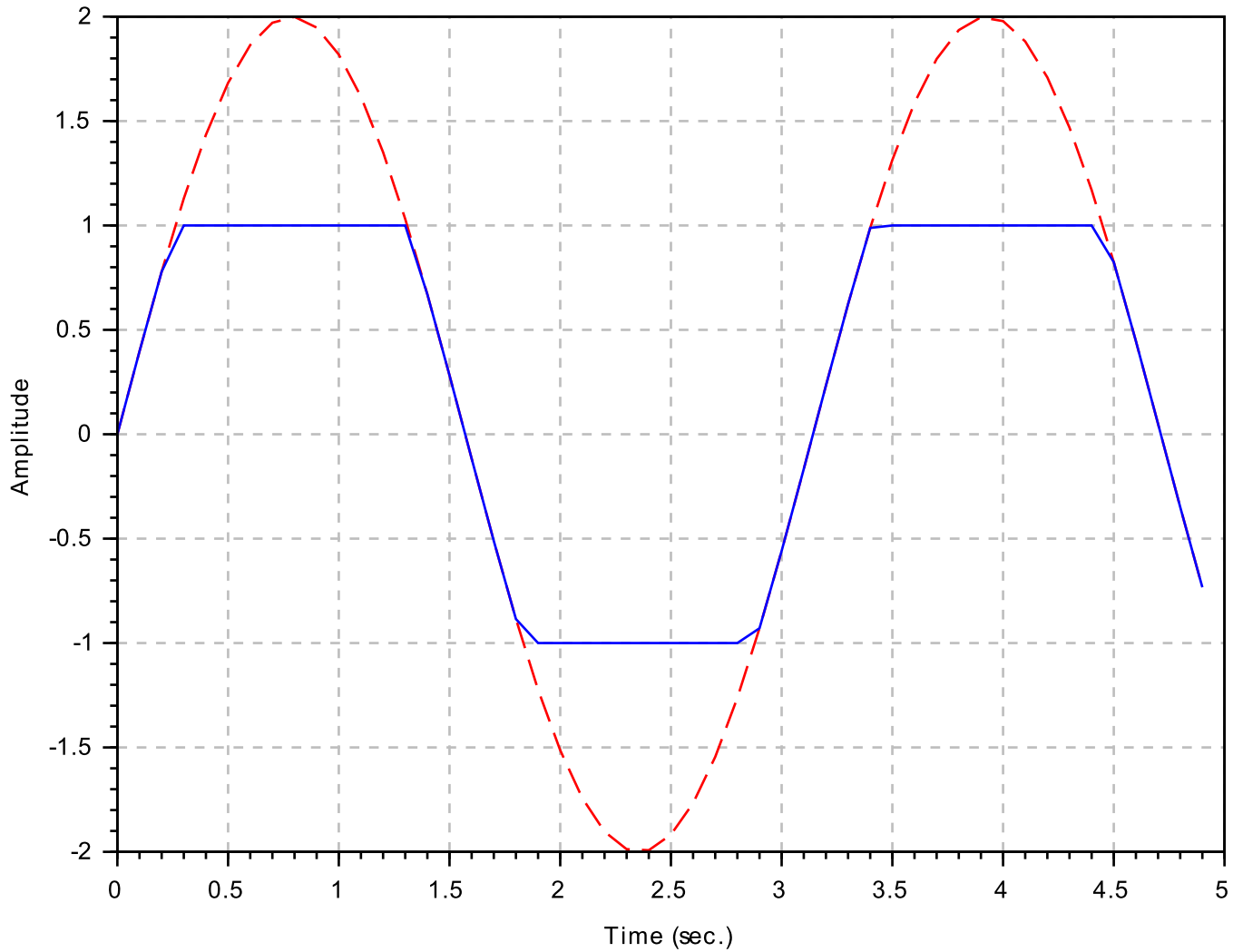
Saturation nonlinearity output to sinusoidal input
