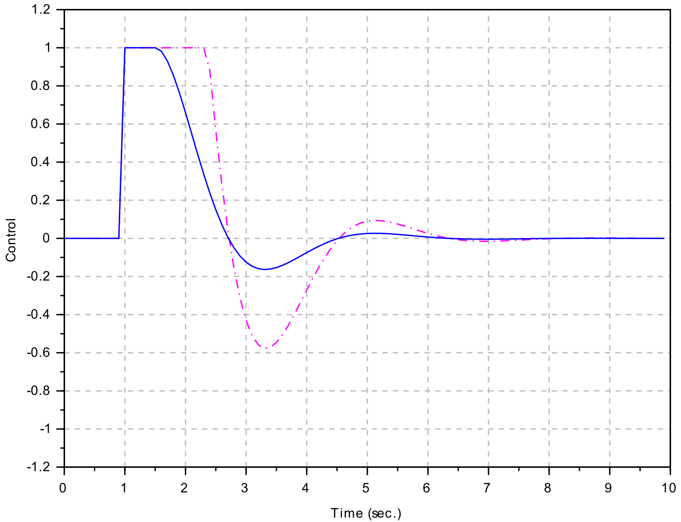
Integrator antiwindup (b) Control effort.
