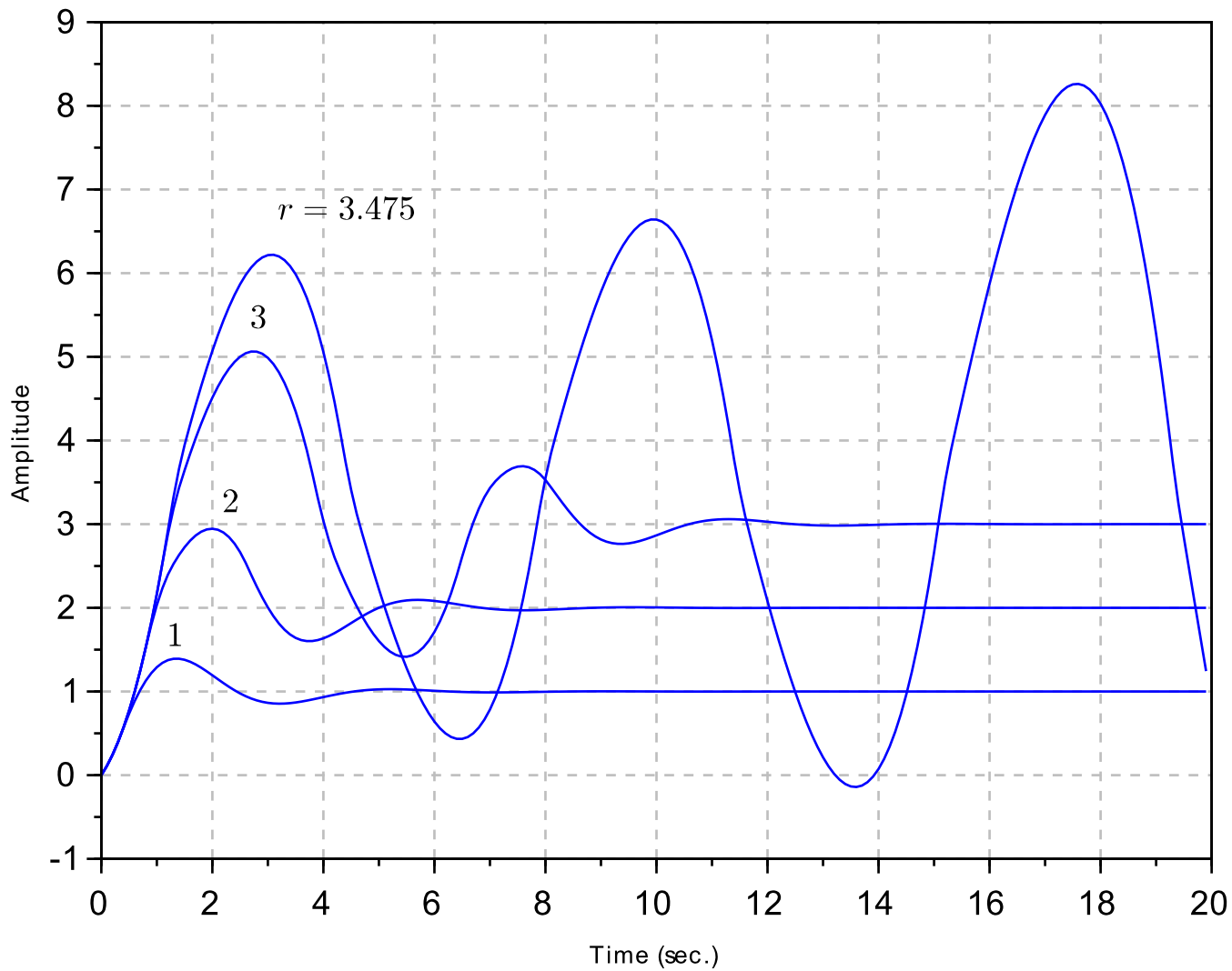
Step response of the system
