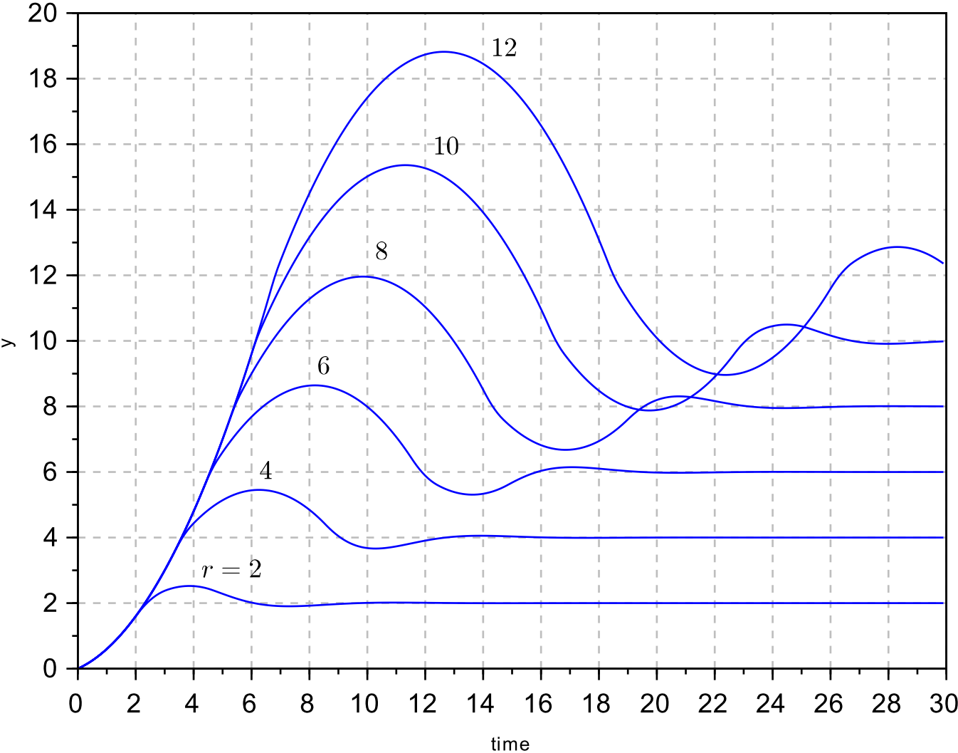
Step response of the system for various input sizes
