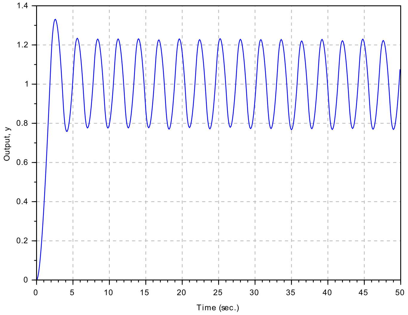
Step response displaying limit cycle oscillations
