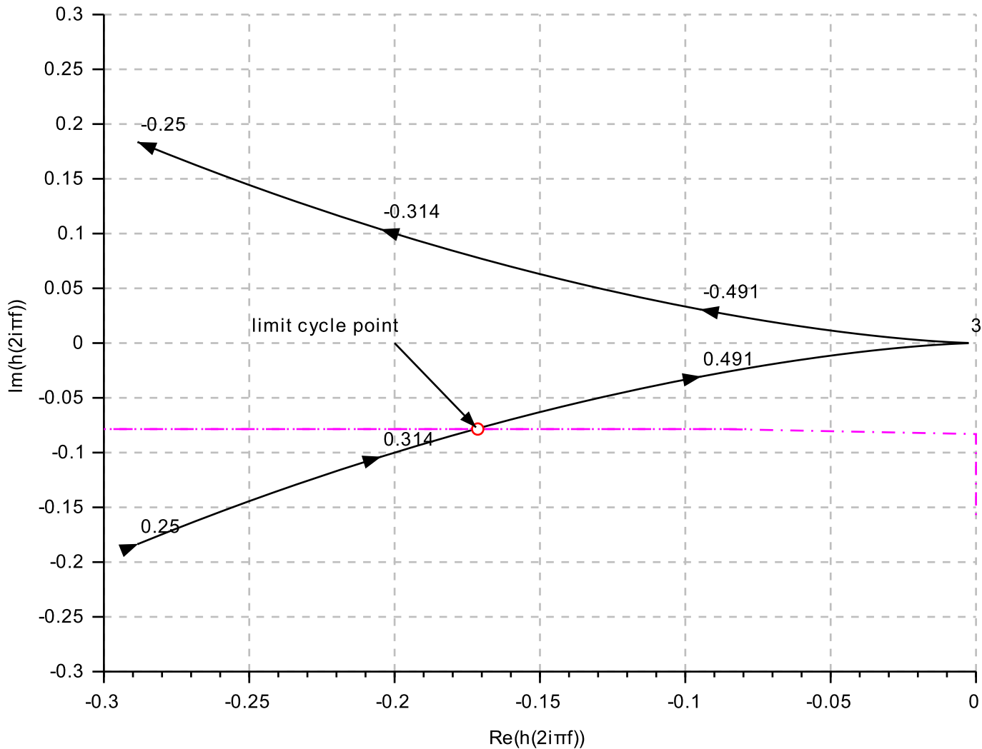
Nyquist plot of system and describing function to determine limit cycle
