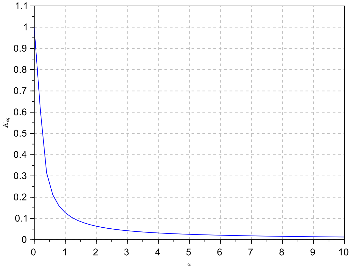
Describing Function for a saturation nonlinearity with N=0.1 and k=1
