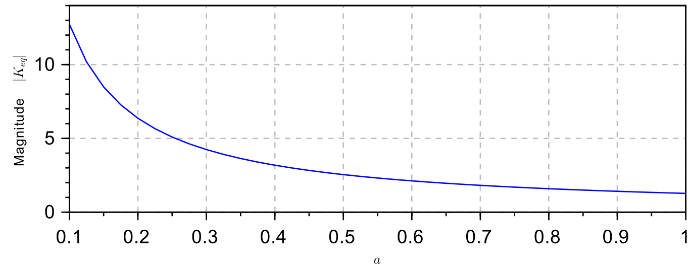
Describing Functin for relay with hysteresis nonlinearity with h=0.1 and N=1
