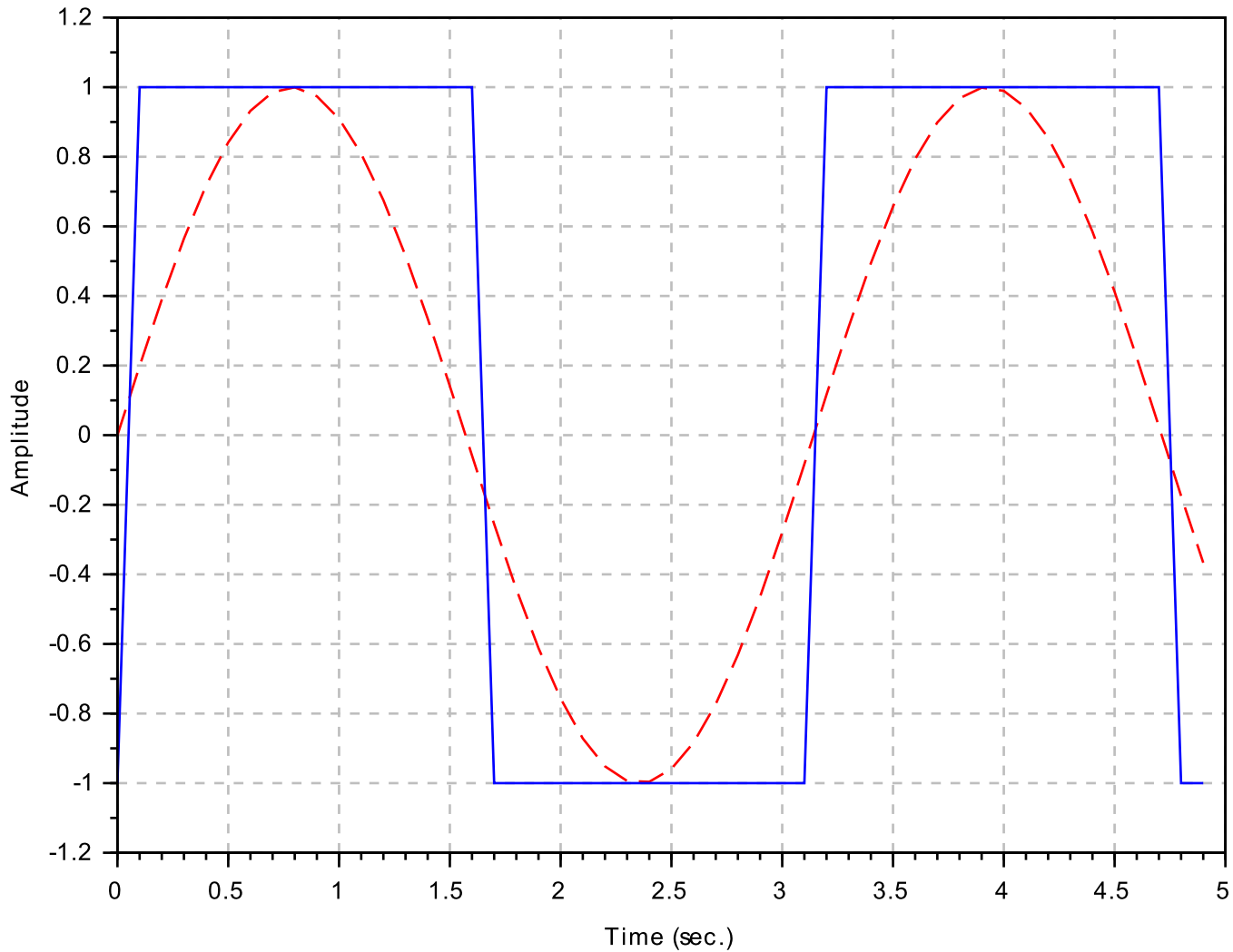
Relay with hysteresis nonlinearity output to sinusoidal input
