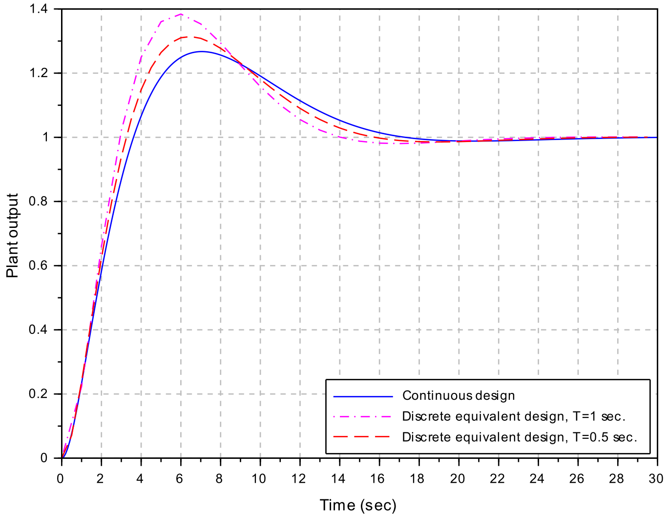
step responses of continous and digital implementations
