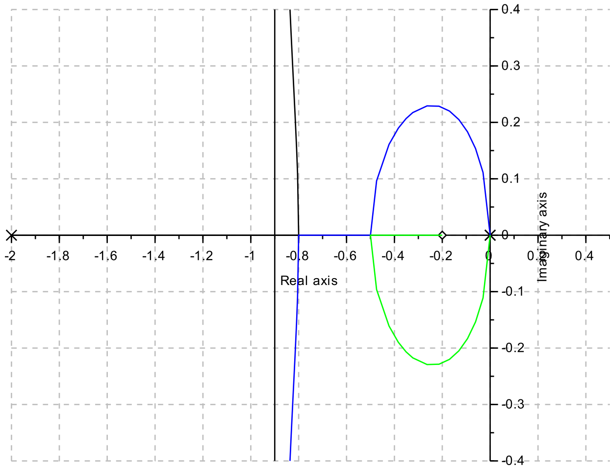
s-plane locus with respect to K
