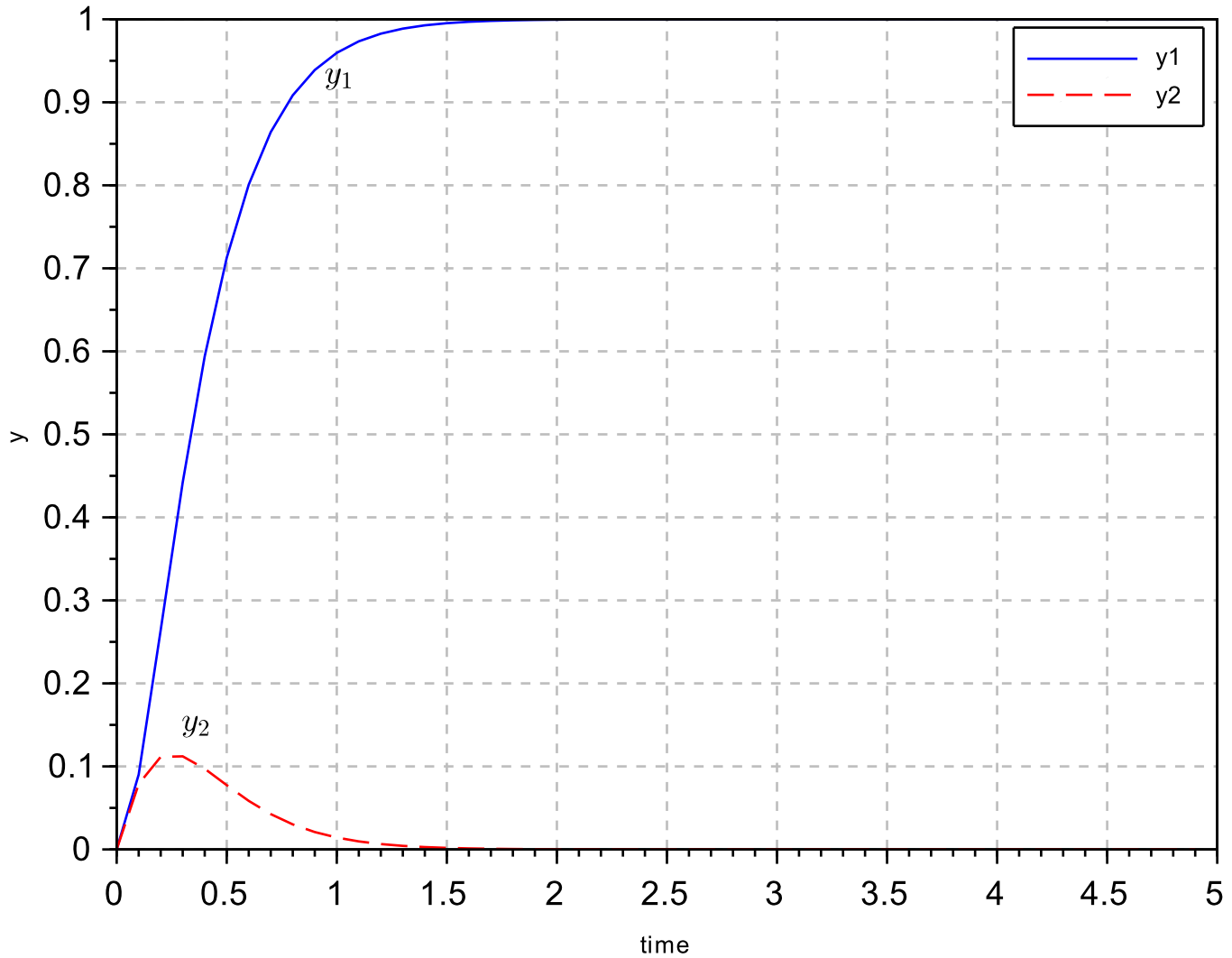
step Response
