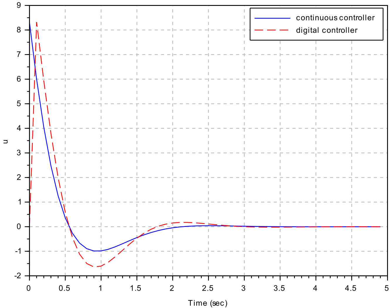
Comaprison of control signals for continuous and discrete controllers
