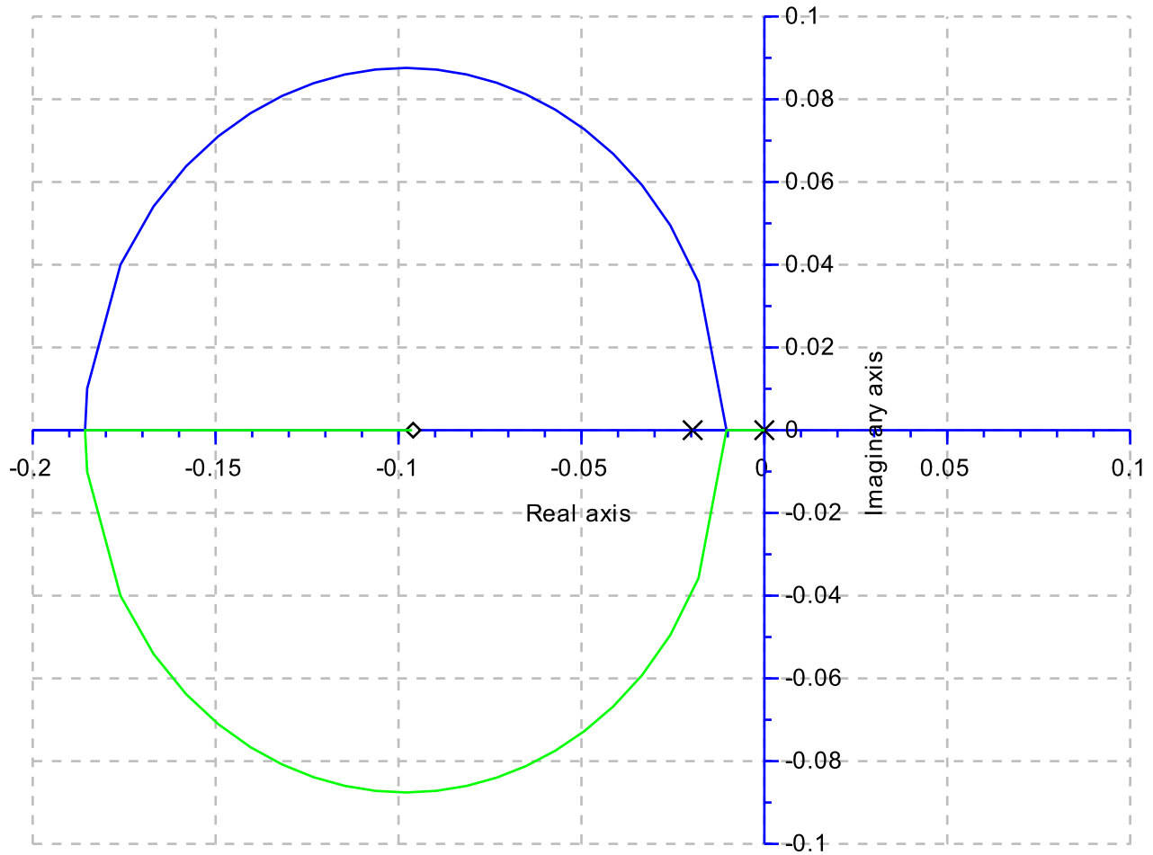
Root locus of lag-lead compensation
