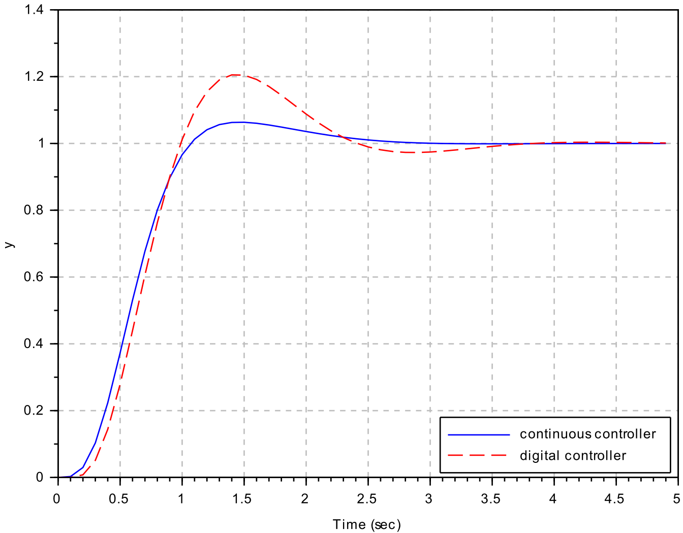
Comaprison of step responses for continuous and discrete controllers
