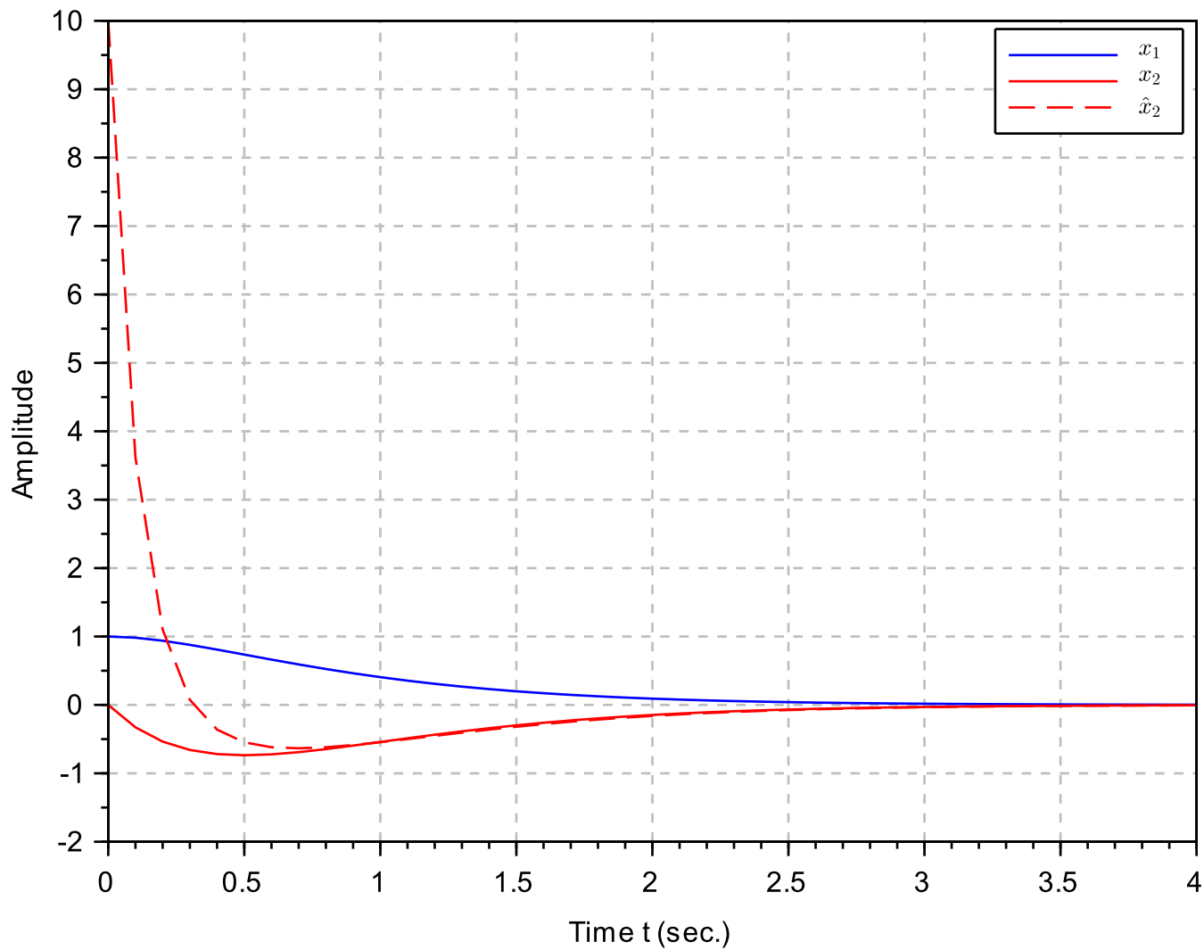
Initial condition response of the reduced order estimator
