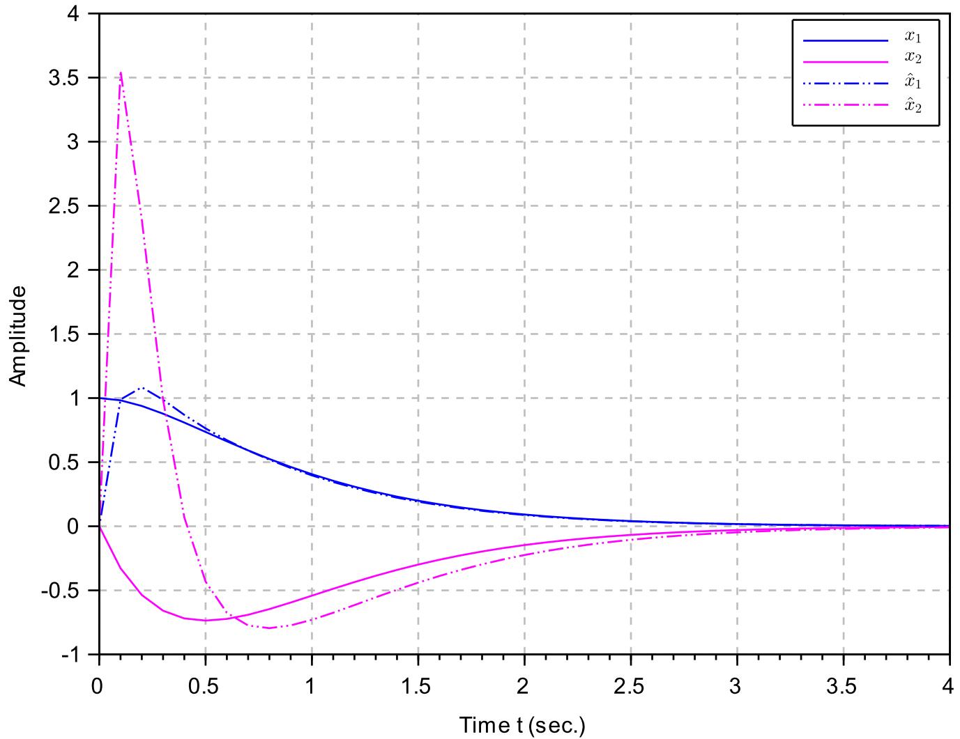
Initial condition response of oscillator showing x and \hat{x}
