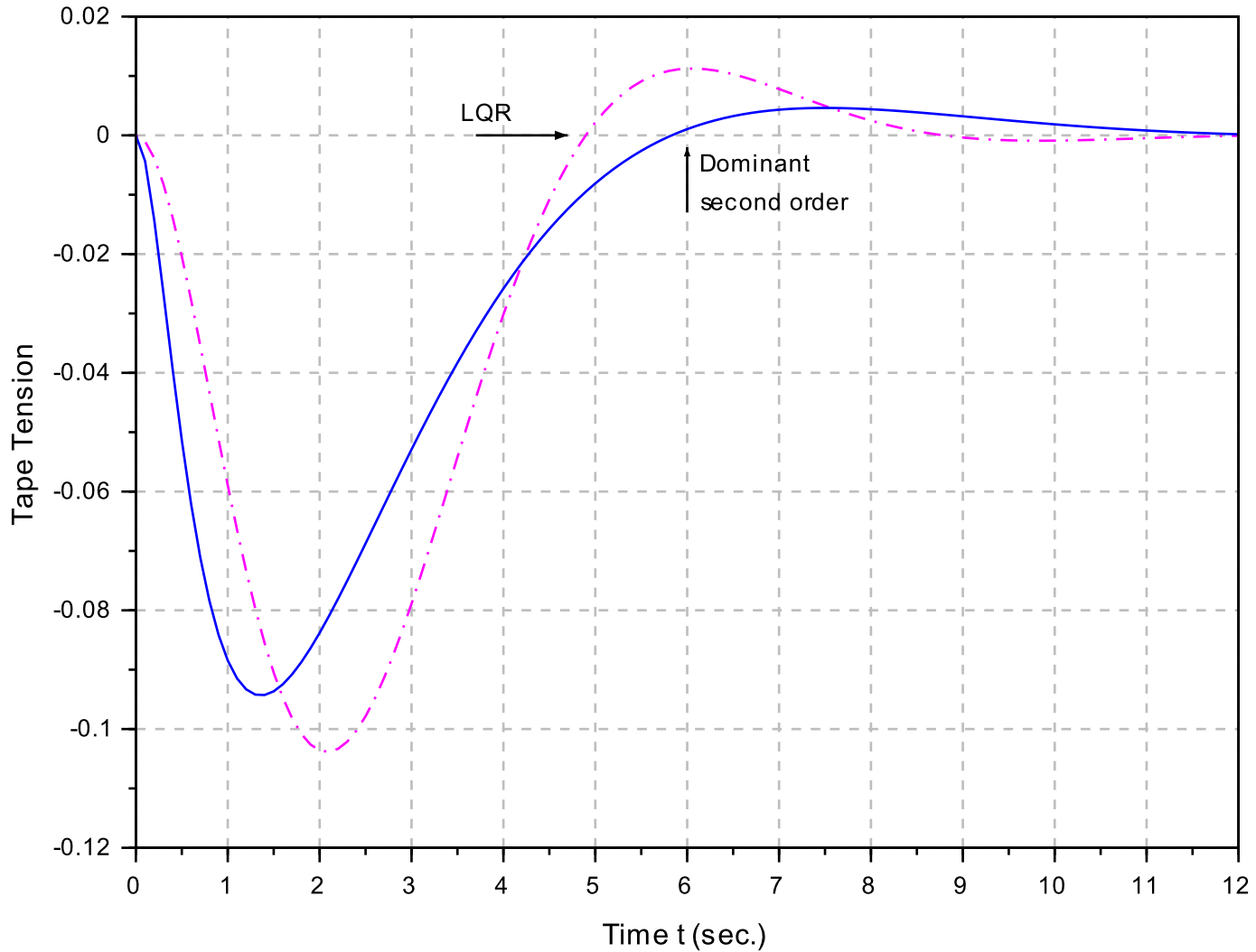
Tension plots for tape servomotor step responses
