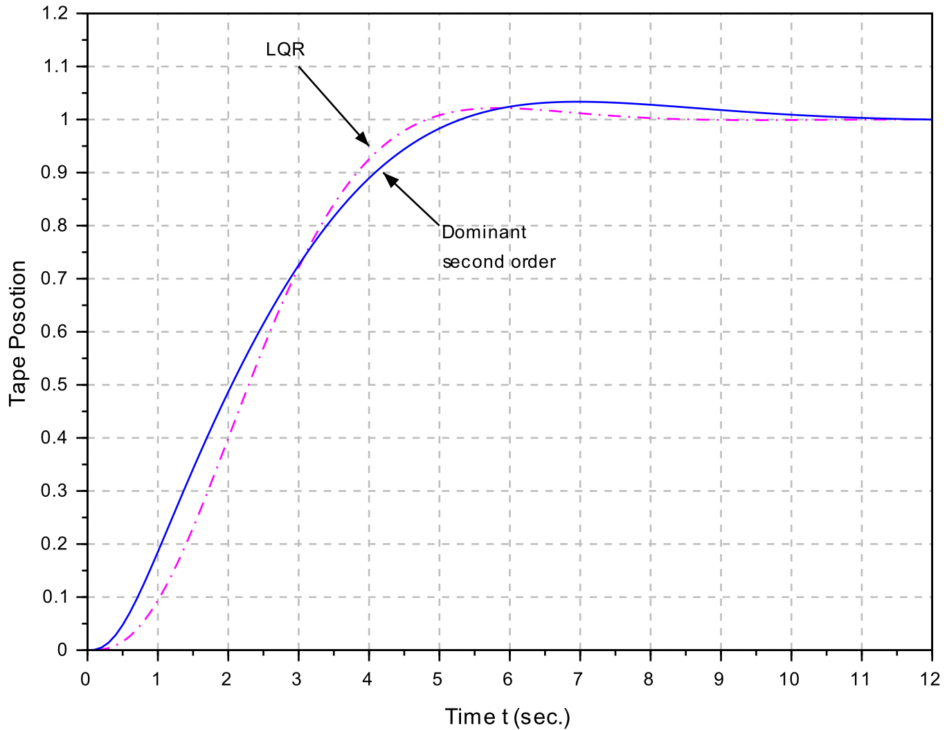
Step response of tape servomotor designs
