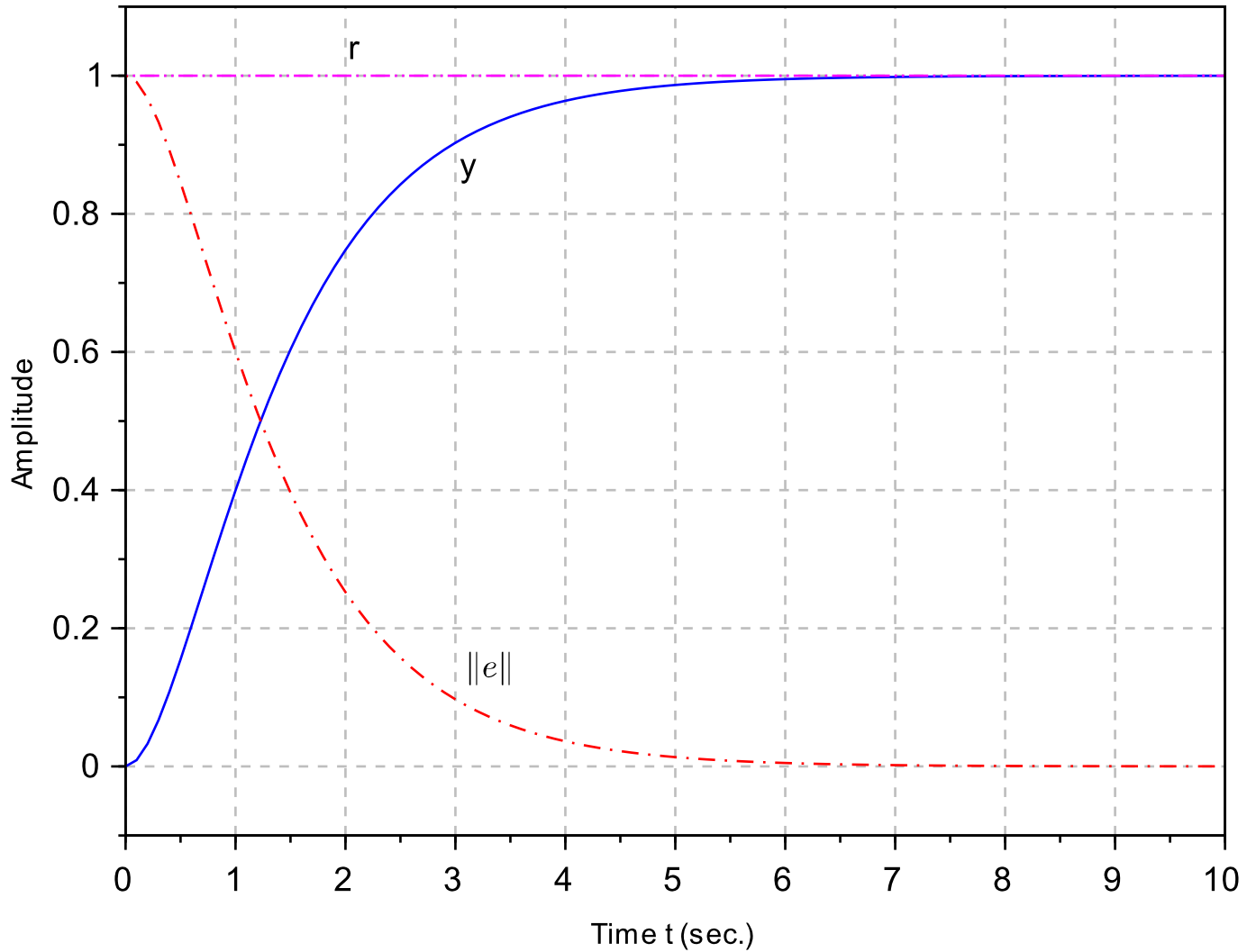
Step response of undamped oscillator to reference input
