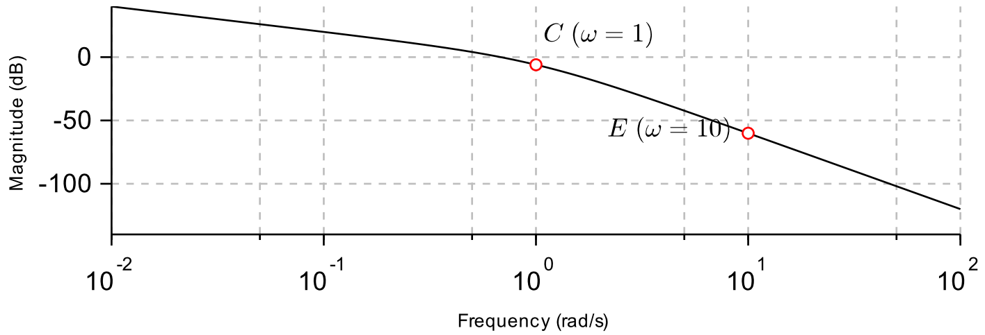
Bode plot for G(s) = 1/[s(s+1)^2]
