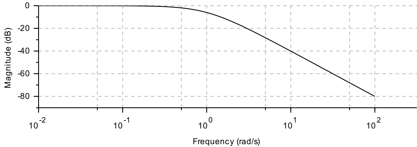
Open loop bode plot for G(s) = 1/(s + 1)^2
