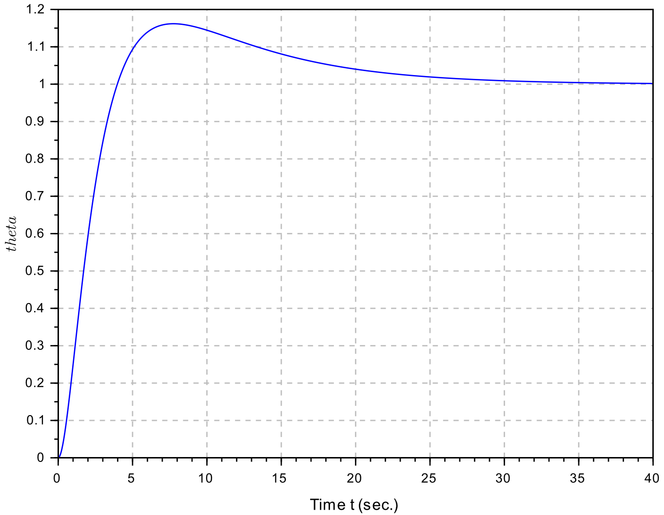
Step response for PID compensation of spacecraft
