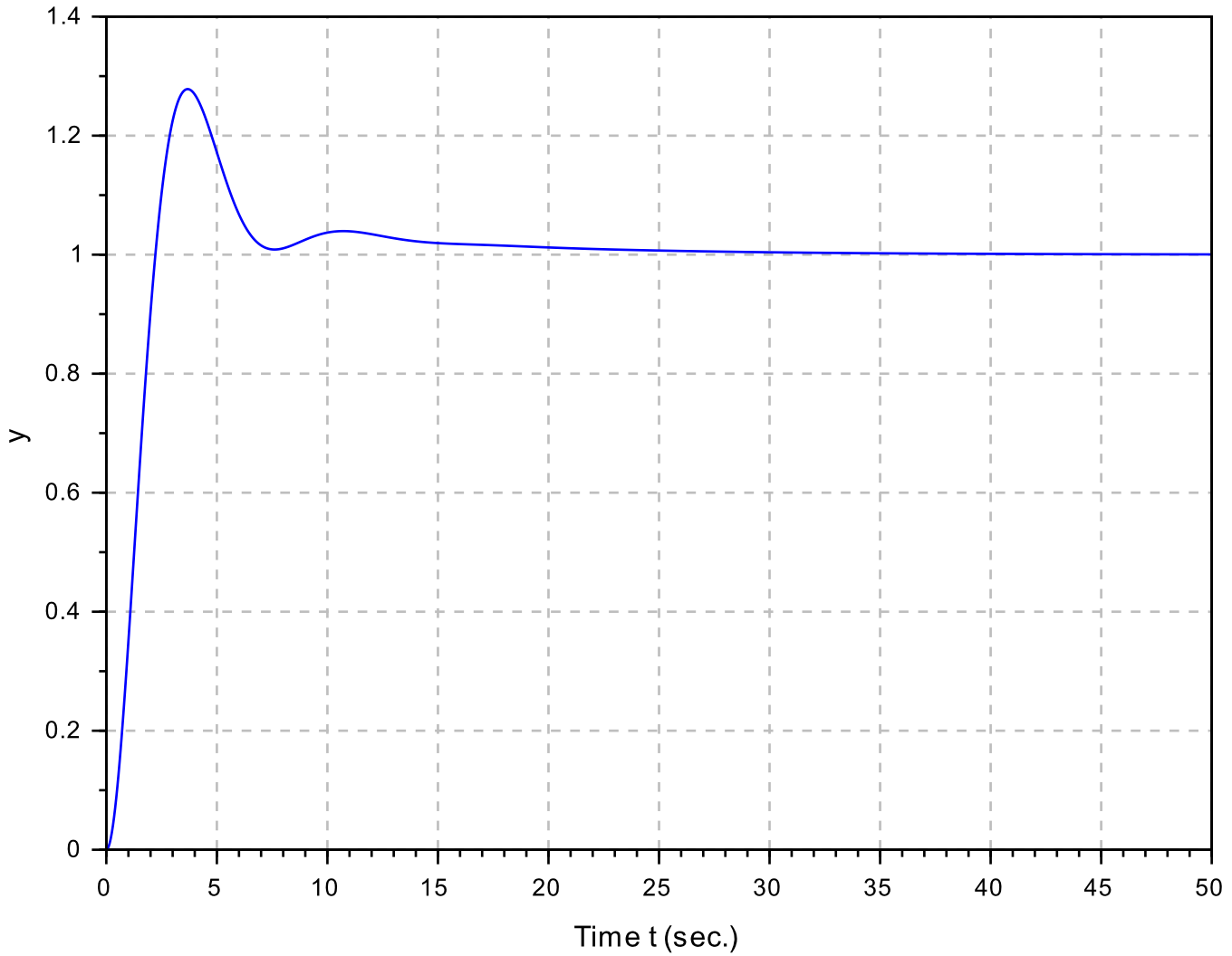
Step response for Lag-compensation design of DC motor
