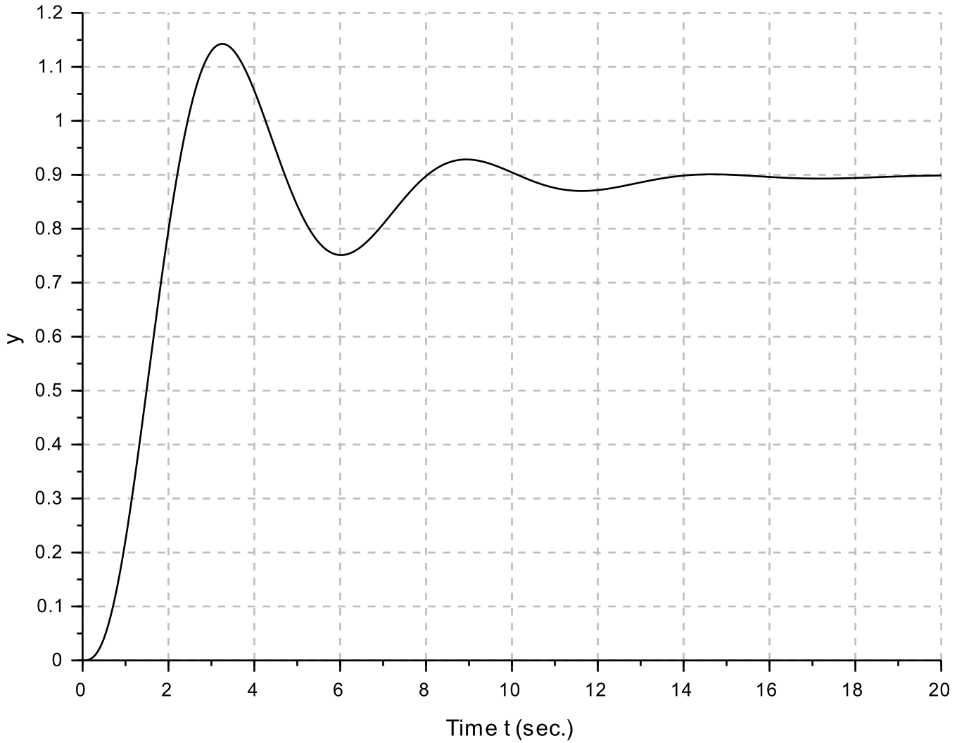
Step response for lag compensation design
