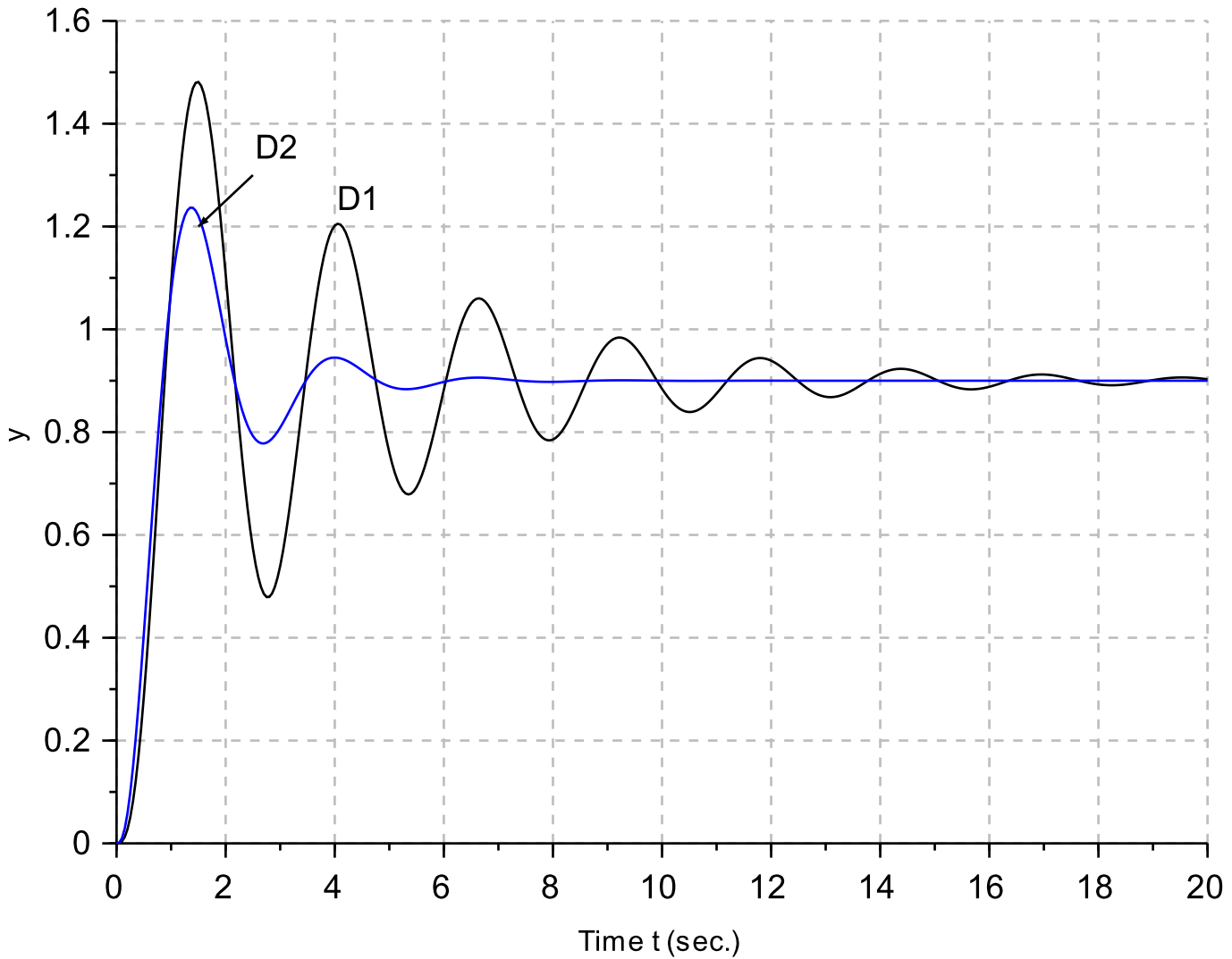
Step response for lead compensation design
