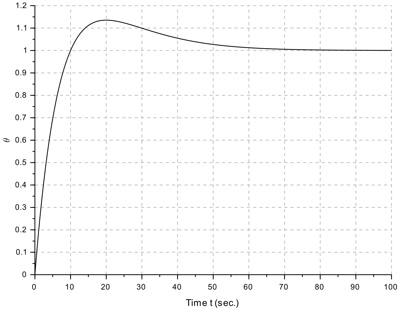
Step response for PD compensation
