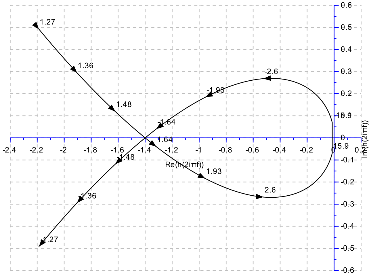
Nyquist plot for G(s) = (s + 10)^2/s^3
