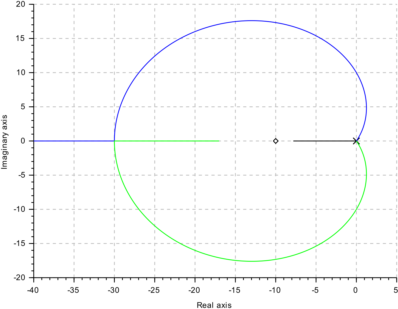
Root locus for G(s) = (s + 10)^2/s^3
