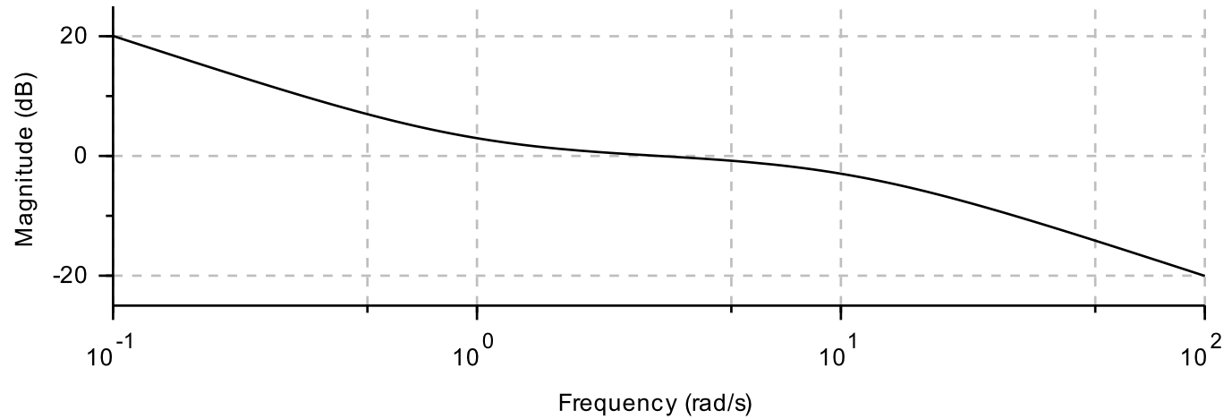
Bode plot for G(s) = (s + 1)/[s(s/10 - 1)]
