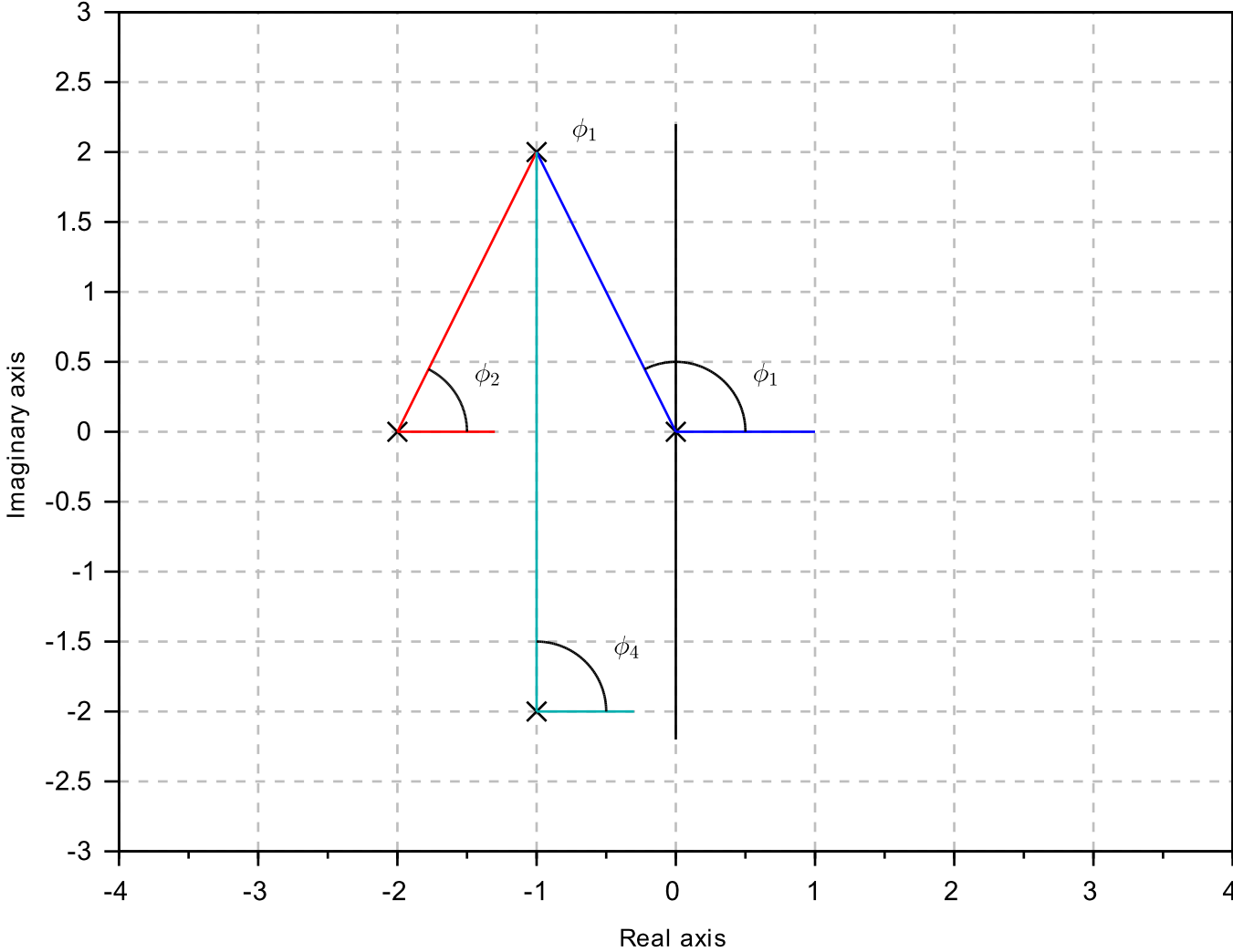
Figure to computing a departure angle for L(s) = \frac{1}{s(s+2)[(s+1)^2+4]}
