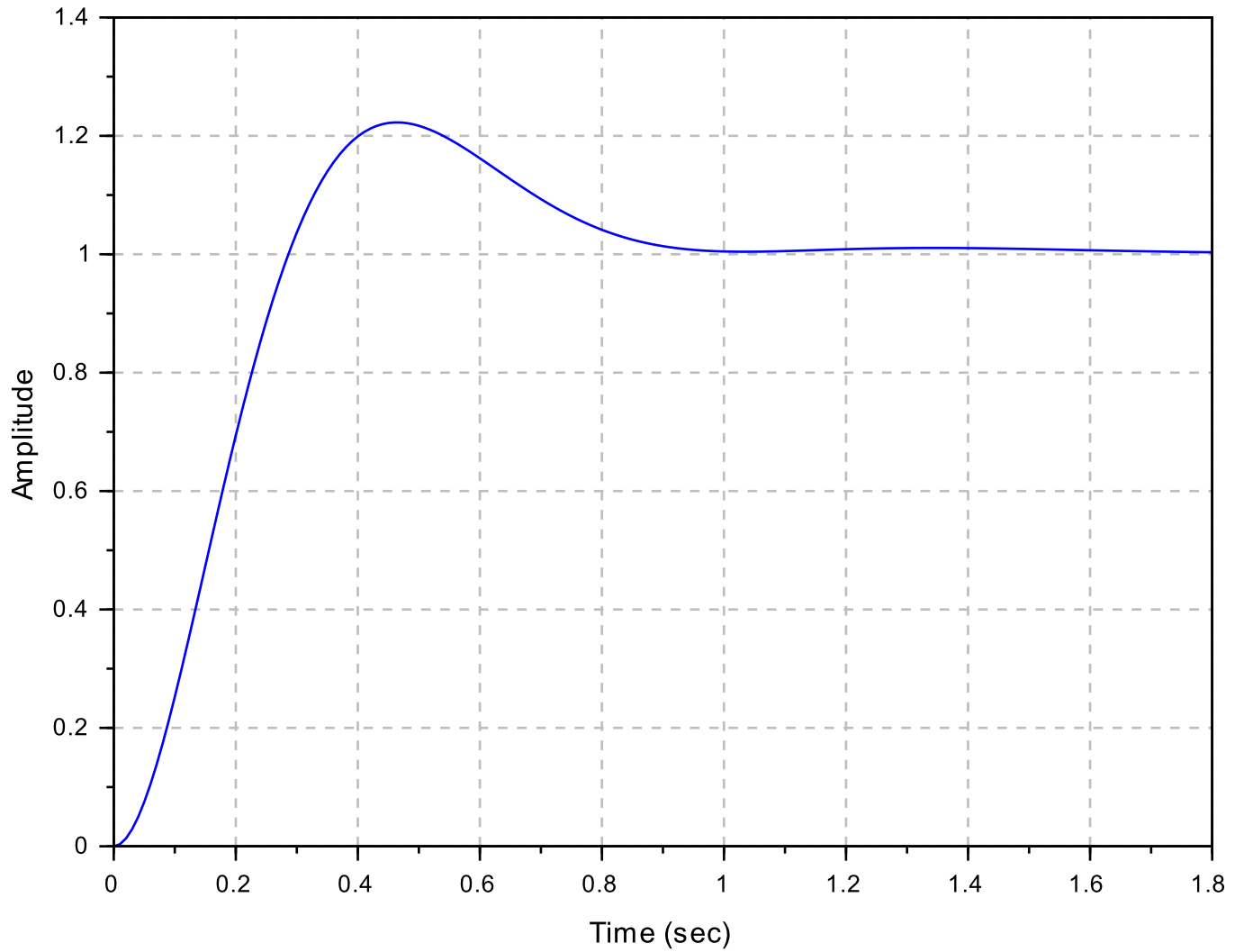
Step response for the system with lead compensator
