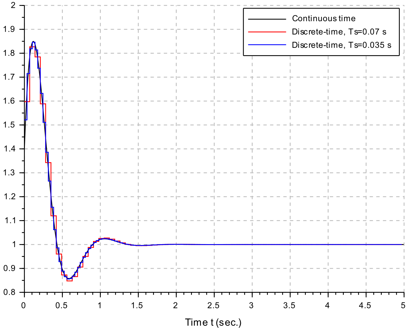
Comparison plots of Speed-control system with continuous and discrete controllers
