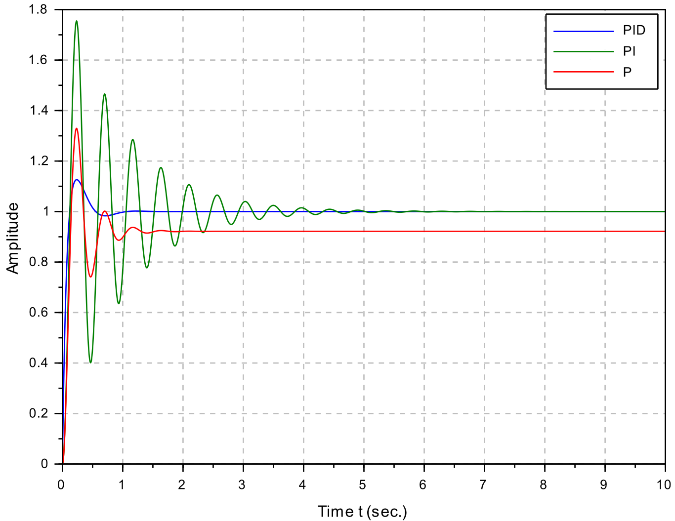
Responses of PID control to step reference input
