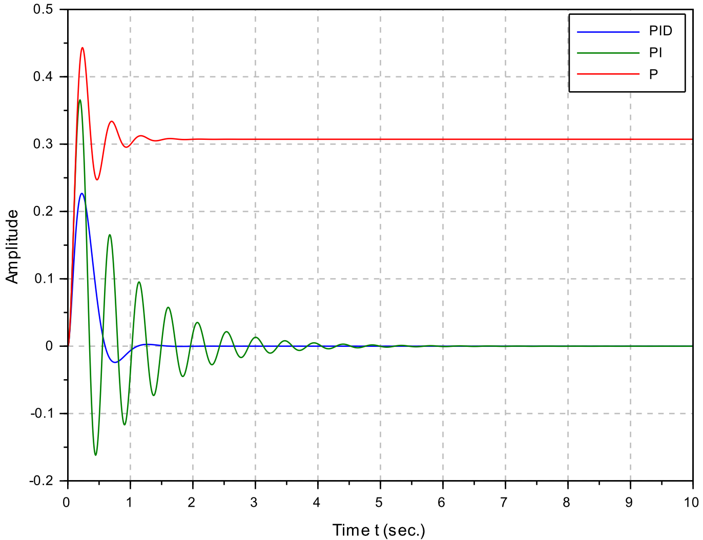
Responses of P,PI and PID control to step disturbance input
