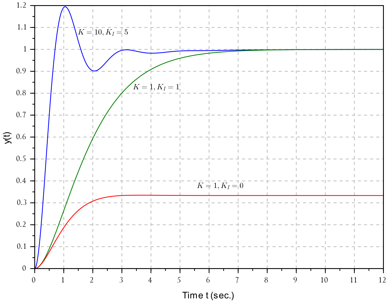
Transient response for the system
