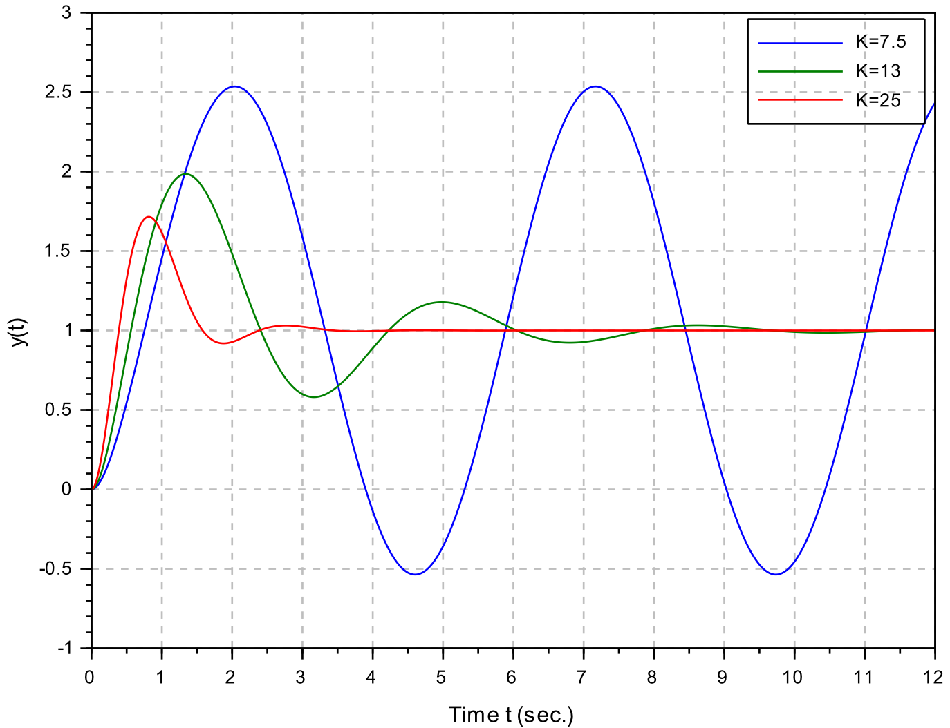
Transient response for different values of K
